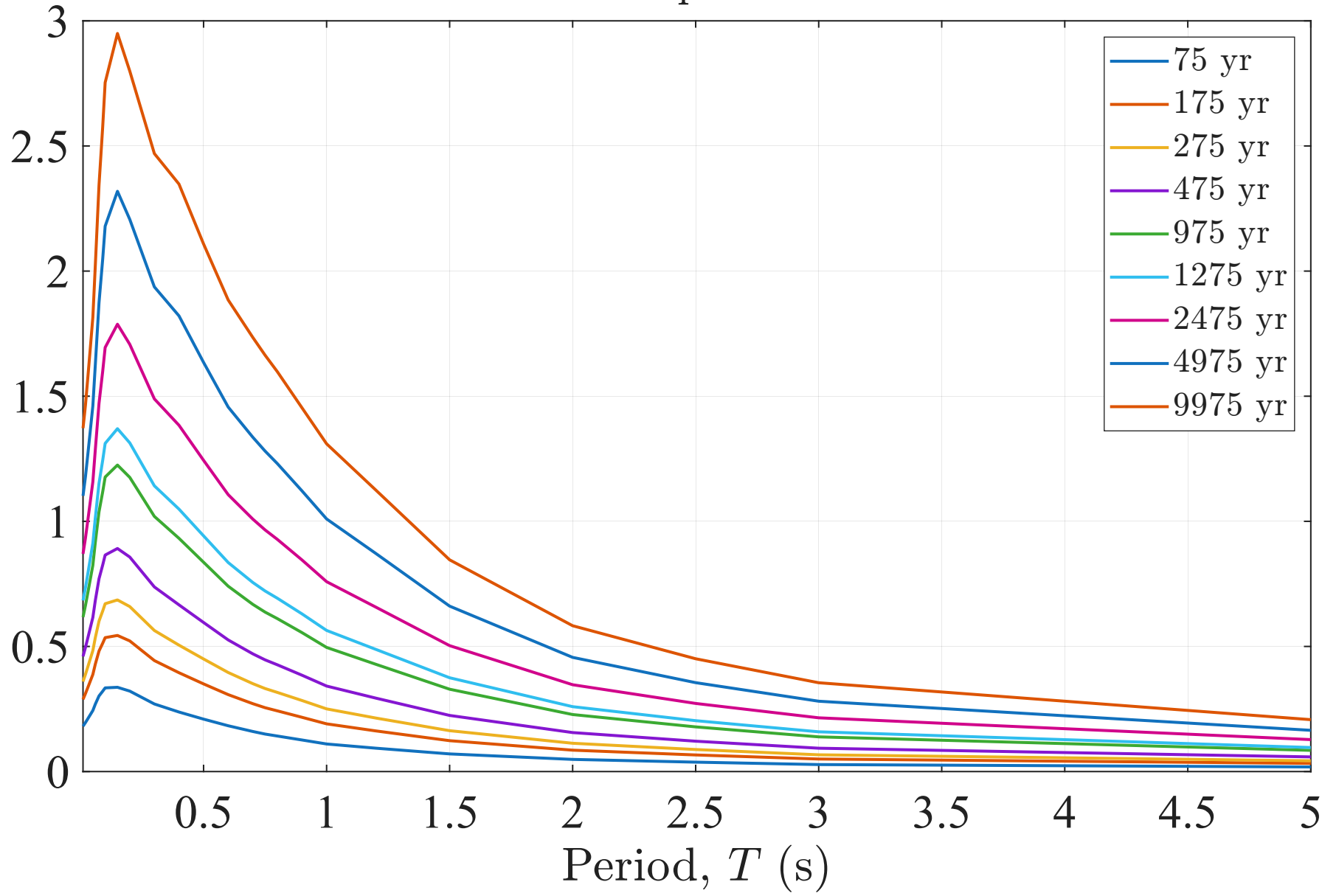
Uniform Hazard Spectrum - Guwahati
